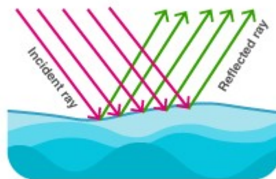
Specular reflection
