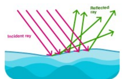
Diffuse reflection
