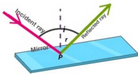
Mirror reflection
